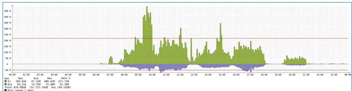
Figure 4. External Bandwidth: 24 hours.
